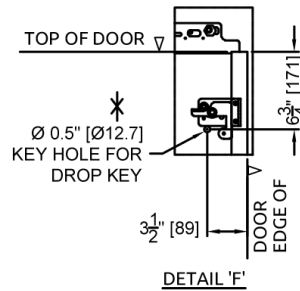
DETAIL 'F'
